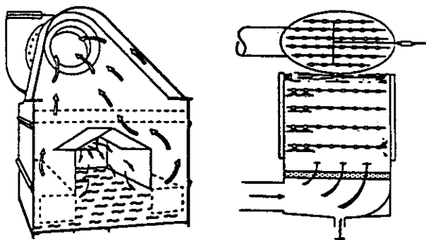
Gambar 4.3 Tipikal Scrubber.
